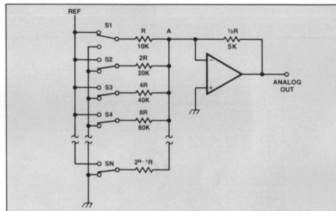
Figure 1. Simplified DAC
